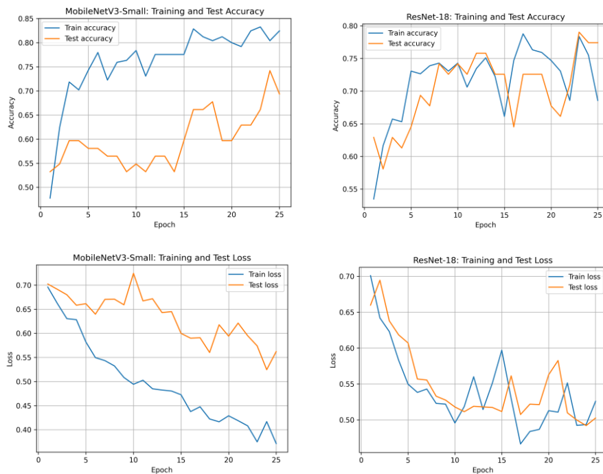
Figure 3. The training curves in Figure 3 demonstrate convergence, as both models show decreasing loss and increasing accuracy over epochs, indicating effective learning without severe overfitting. However, there is a slight divergence between training and testing
